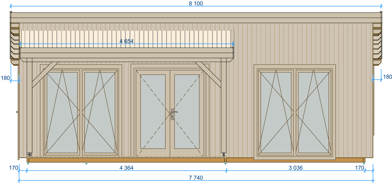
Front Elevation
