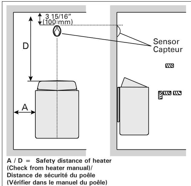
Figure 9. The place of the temperature sensor of the control unit in connection with wall-mounted heaters
