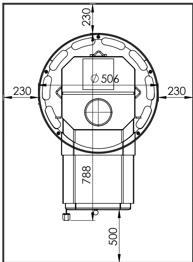
Minimum distance to wall
